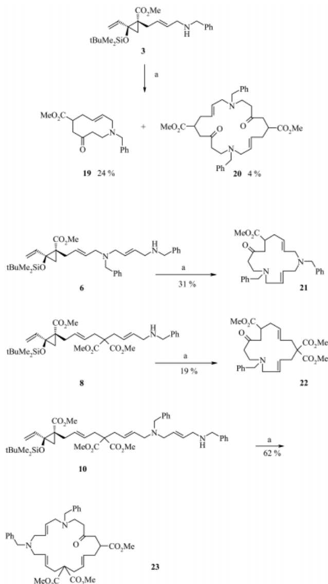
Scheme 4. a) CsF, TEBA, DMF, 90 °C, 22–25 h
