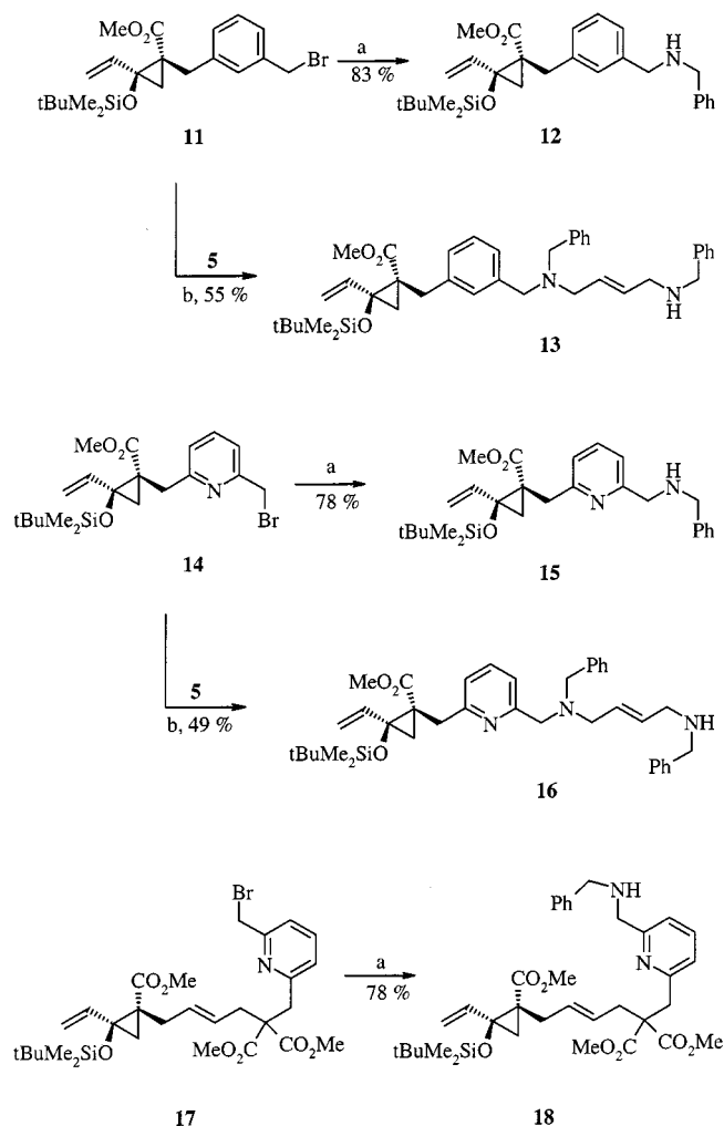
Scheme 3. a) PhCH 2 NH 2 , CH 2 Cl 2 , room temp., 3 h; b) K 2 CO 3 , CH 3 CN, room temp. to reflux, 24 h
