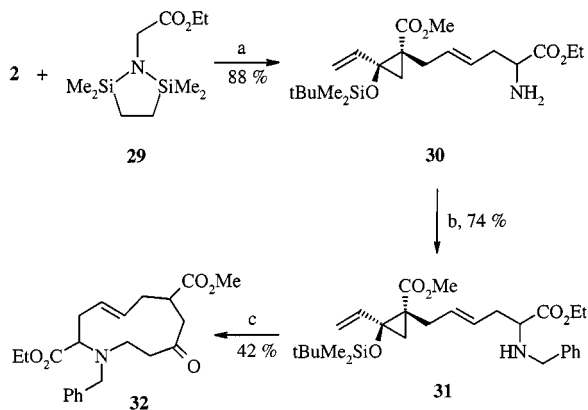
Scheme 6. a) i. LDA, -78^{\circ}\text{C} , ii. Silica gel; b) i. PhCHO, \text{MgSO}_4 , ii. \text{NaBH}_4 , MeOH, room temp.; c) CsF, TEBA, DMF, 90^{\circ}\text{C} , 25 h
