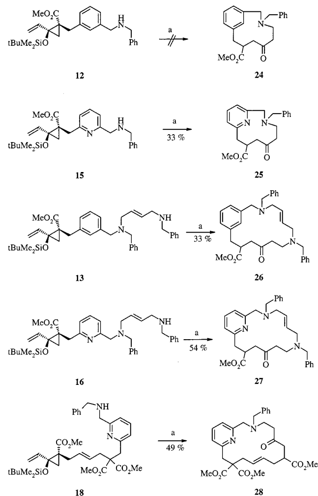
Scheme 5. a) CsF, TEBA, DMF, 90 °C, 22–25 h
