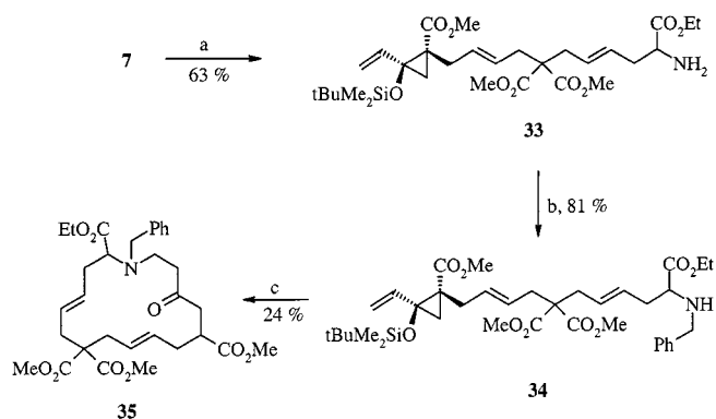
Scheme 7. a) i. 29 , LDA, -78^{\circ}\text{C} , ii. silica gel; b) i. PhCHO, \text{MgSO}_4 , ii. \text{NaBH}_4 , MeOH, room temp.; c) CsF, TEBA, DMF, 90^{\circ}\text{C} , 28 h
