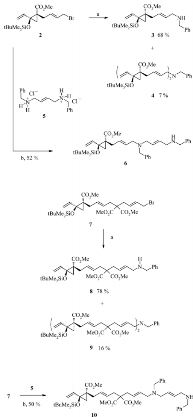
Scheme 2. a) PhCH 2 NH 2 , CH 2 Cl 2 , room temp., 3 h; b) K 2 CO 3 , CH 3 CN, room temp. to reflux, 24 h
